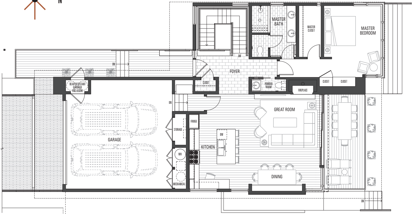
Main Floor
