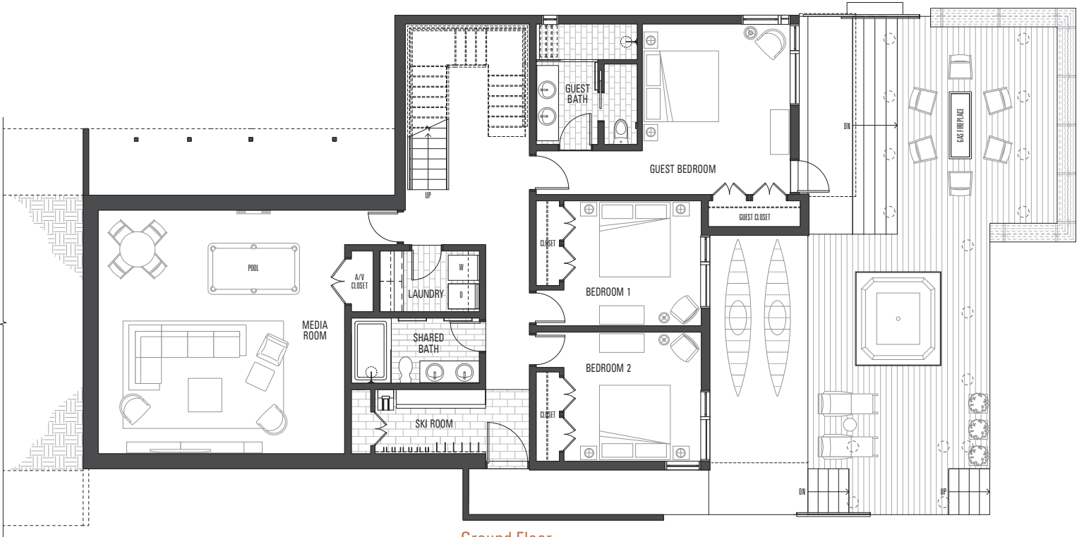
Ground Floor
